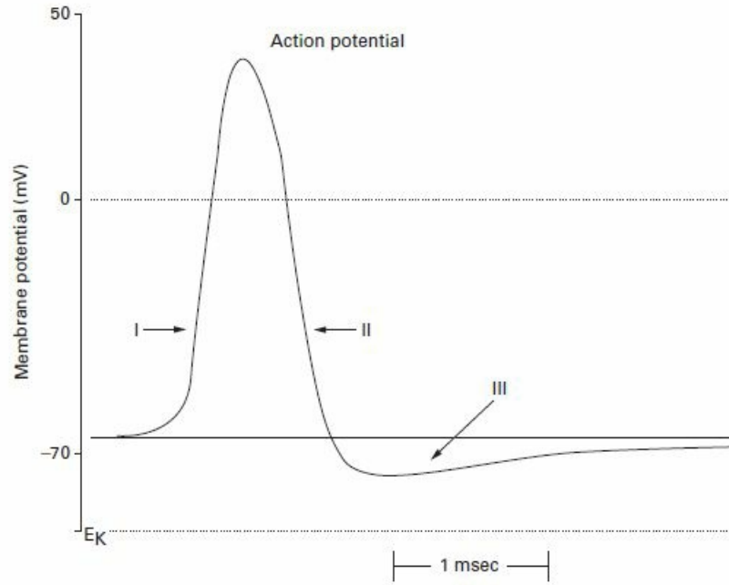
Figure 11.1 A schematic drawing of an action potential indicating the main features of the changing voltage across the cell membrane: (I) a rapid rise of V_m , followed by (II) a steep decline to values below that of the resting potential and (III) an extended refractory period. (Craver 2007, 50; by permission of Oxford University Press)
