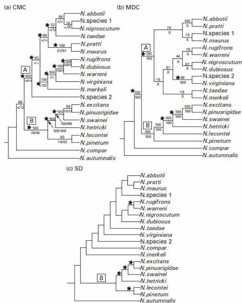
Figure 5.1 Three phylogenetic trees of the sawfly (genus Neodiprion ). The different trees result from different methods applied to a single data set. Although seemingly a normal science, phylogenetics, like many disciplines, sustains continued debates over the relative merits of
