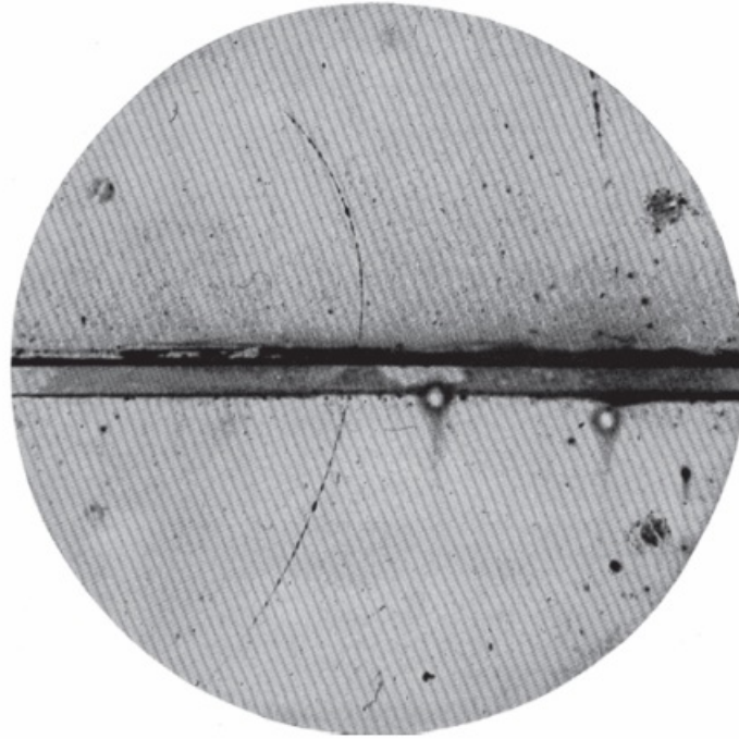
Figure 10.1 A cloud chamber photograph of a track left by a positron. The particle enters from below and passes through a 6 mm lead plate across the center. The subsequent loss of momentum results in the greater curvature of the track in the upper region. (Reprinted with permission from Carl Anderson, “The positive electron.” Physical Review 43, 492 (1933). Copyright 1933 by the American Physical Society.)
