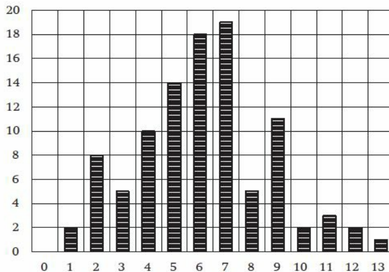
Figure 9.2 Dice game results, N = 100
