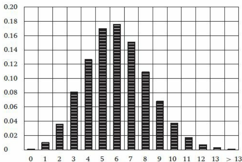
Figure 9.1 The binomial distribution for Y_i ( p = 1/6 , N = 36 ).
