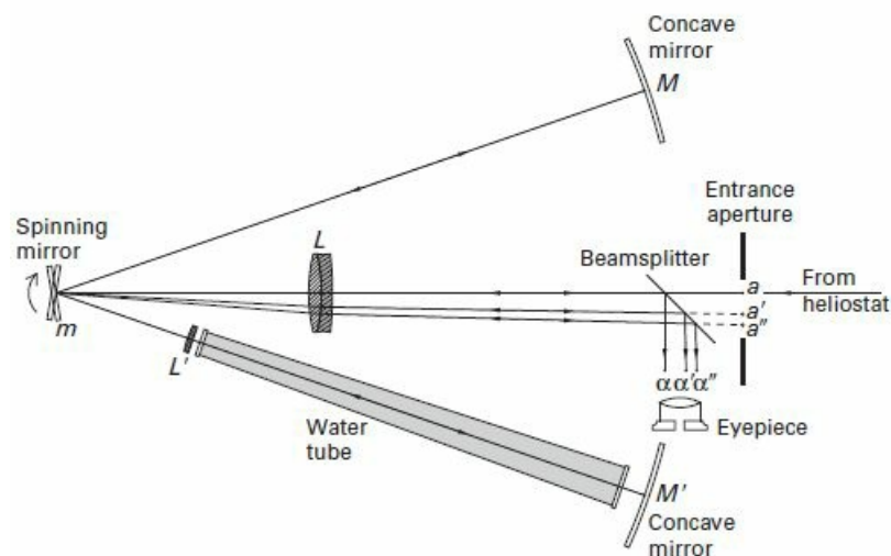
Figure 3.1 Foucault's experimental arrangement. (From Tobin, 2003, 125. Image courtesy of William Tobin.)
